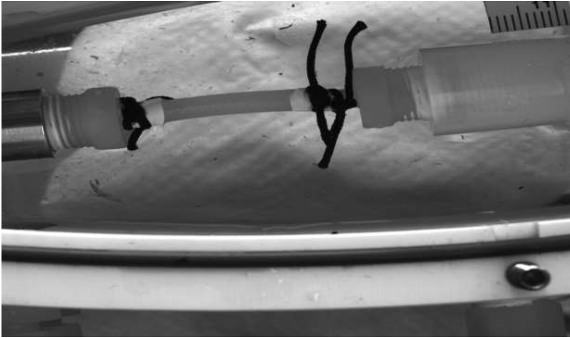
Figure 5.7. Experimental setup of burst pressure on the fabricated tube.
